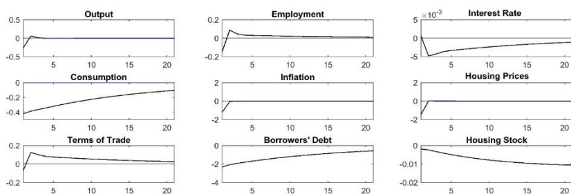
Figure 6 Impulse Responses
